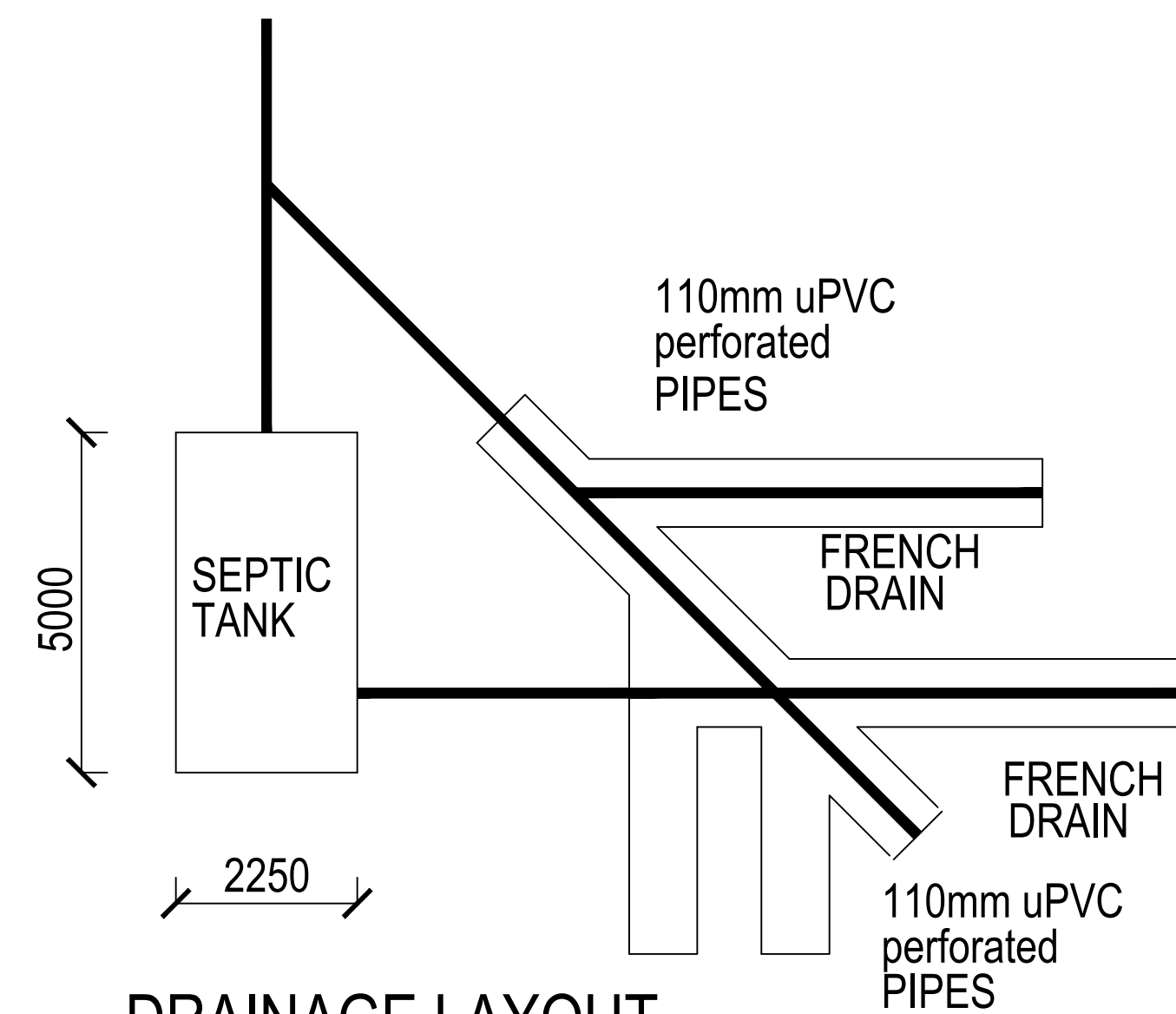
DRAINAGE LAYOUT
