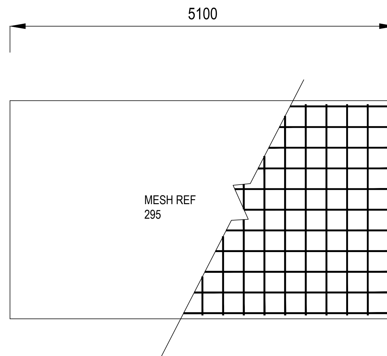
FLOOR SLAB REINFORCEMENT
